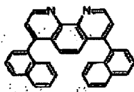
Structural formula 9:
